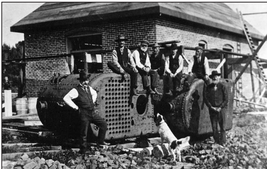
Above – Working on the chimney of the Seul Choix fog signal building. Note the two whistle fog signals on either side of the chimney. Photo courtesy of the author. Below – Workers install a boiler for a steam-powered fog signal. Lighthouse Society photo.
